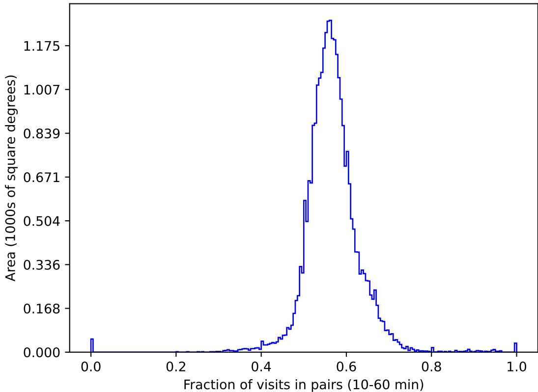
baseline_v3.3_10yrs gri All sky: Fraction of visits in pairs (10-60 min)
