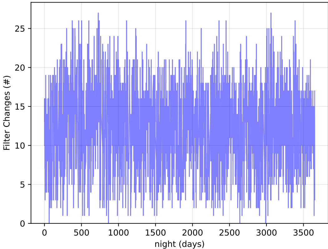
baseline_v3.3_10yrs Per Night: Filter Changes
