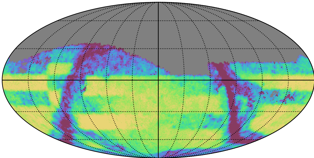
baseline_v3.3_10yrs Yr 3-4 z band: Exgal_CoaddM5
