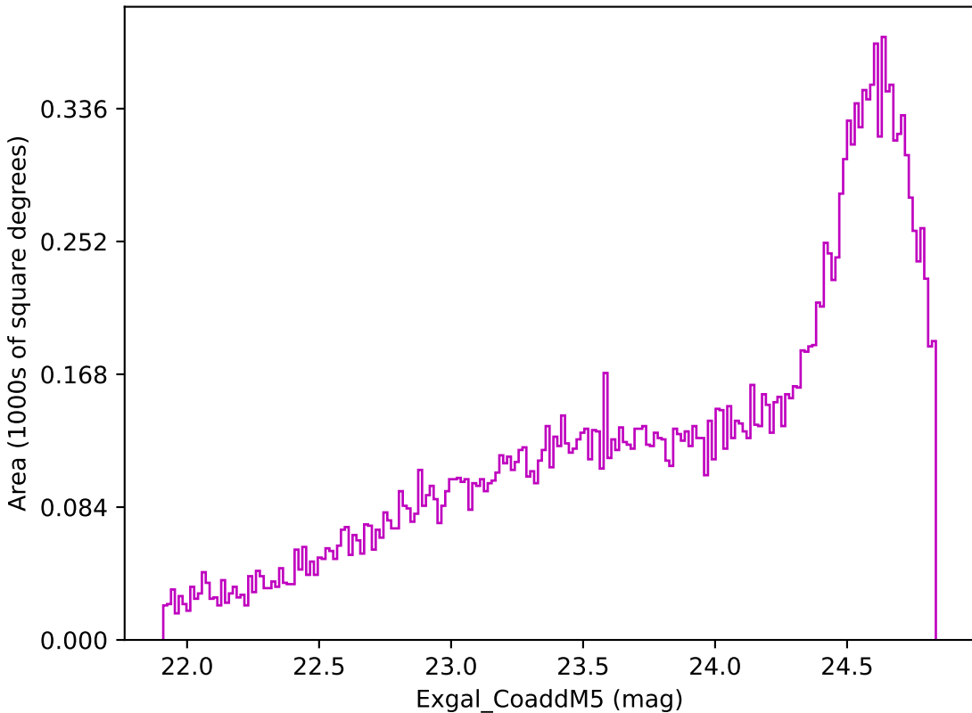
baseline_v3.3_10yrs Yr 3-4 z band: Exgal_CoaddM5
