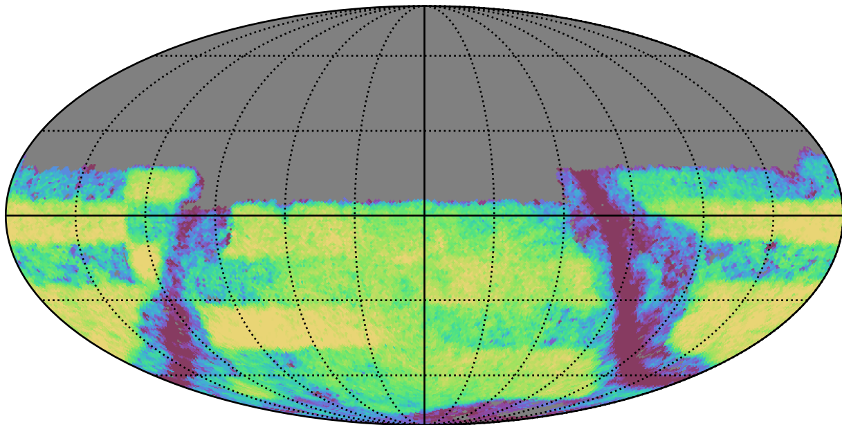
baseline_v3.3_10yrs Yr 3-4 y band: Exgal_CoaddM5
