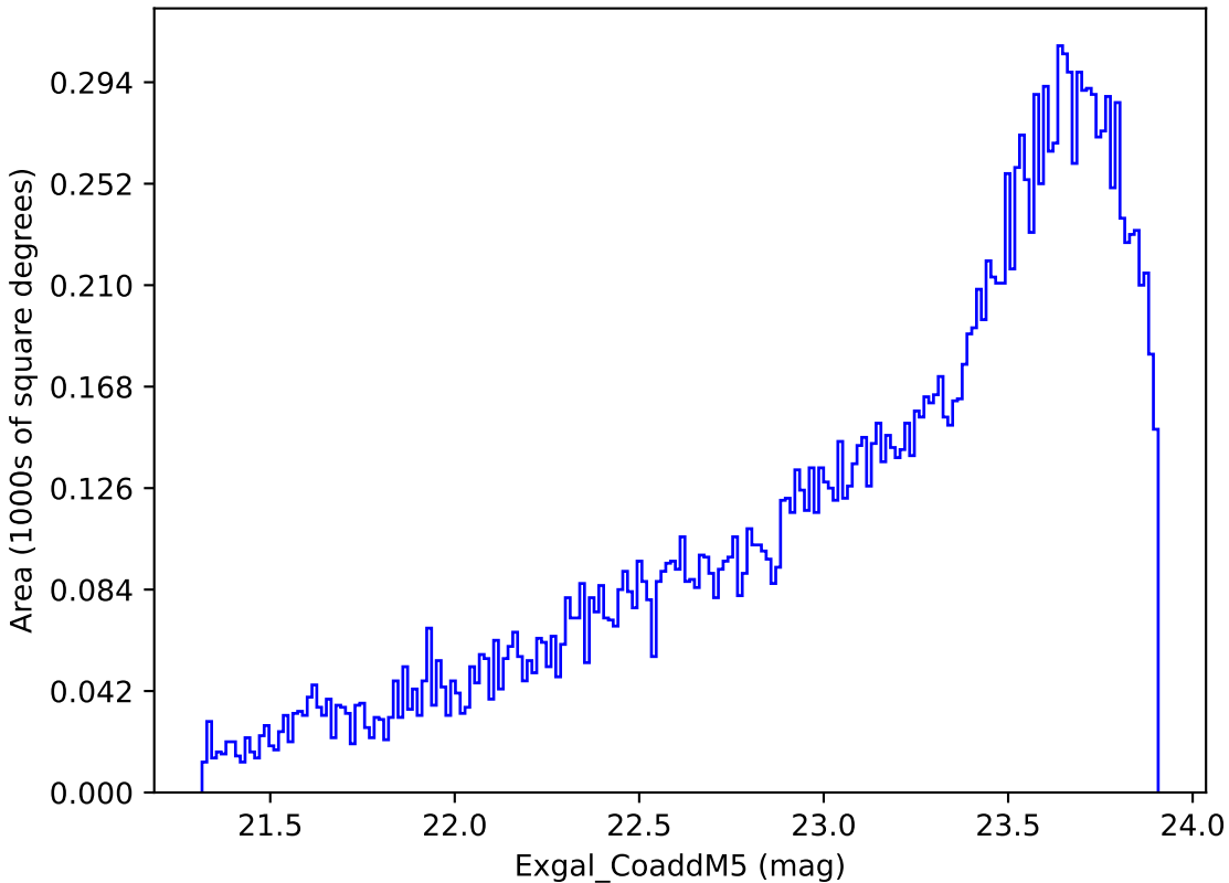
baseline_v3.3_10yrs Yr 3-4 y band: Exgal_CoaddM5
