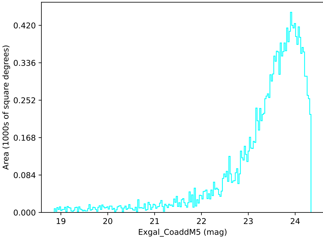
baseline_v3.3_10yrs Yr 3-4 u band: Exgal_CoaddM5
