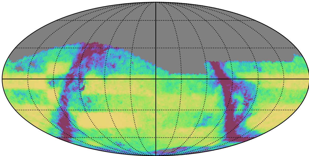
baseline_v3.3_10yrs Yr 3-4 r band: Exgal_CoaddM5
