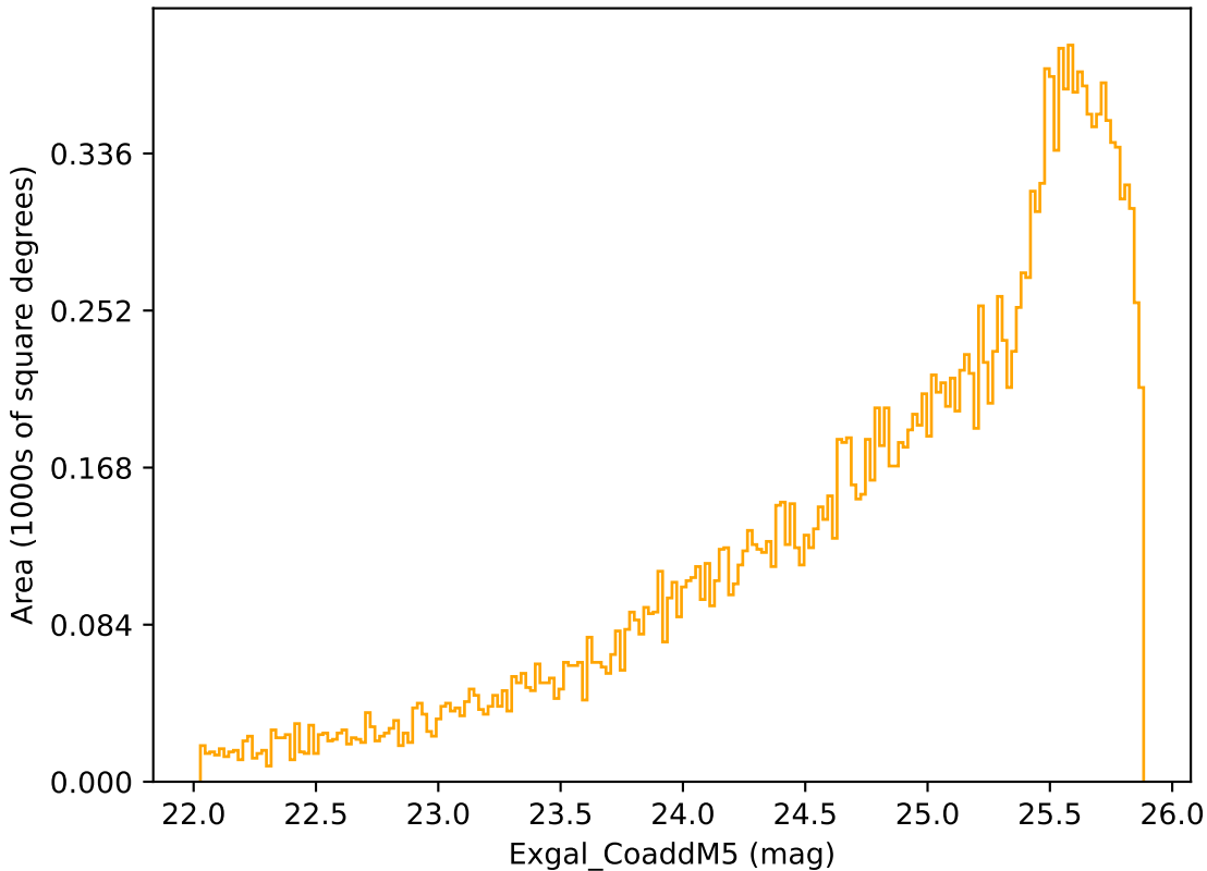
baseline_v3.3_10yrs Yr 3-4 r band: Exgal_CoaddM5
