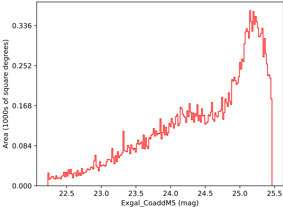
baseline_v3.3_10yrs Yr 3-4 i band: Exgal_CoaddM5
