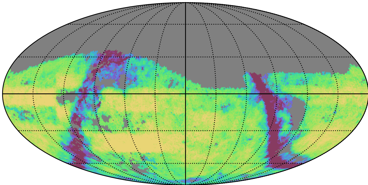
baseline_v3.3_10yrs Yr 3-4 g band: Exgal_CoaddM5
