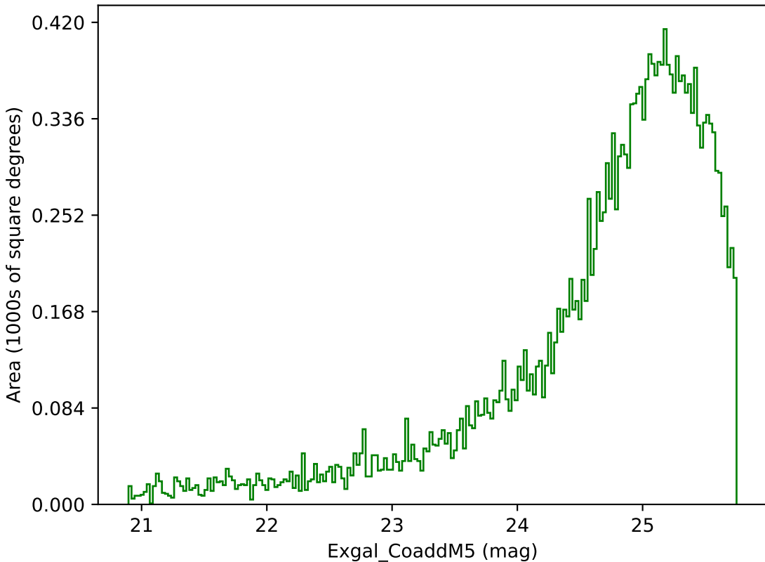
baseline_v3.3_10yrs Yr 3-4 g band: Exgal_CoaddM5
