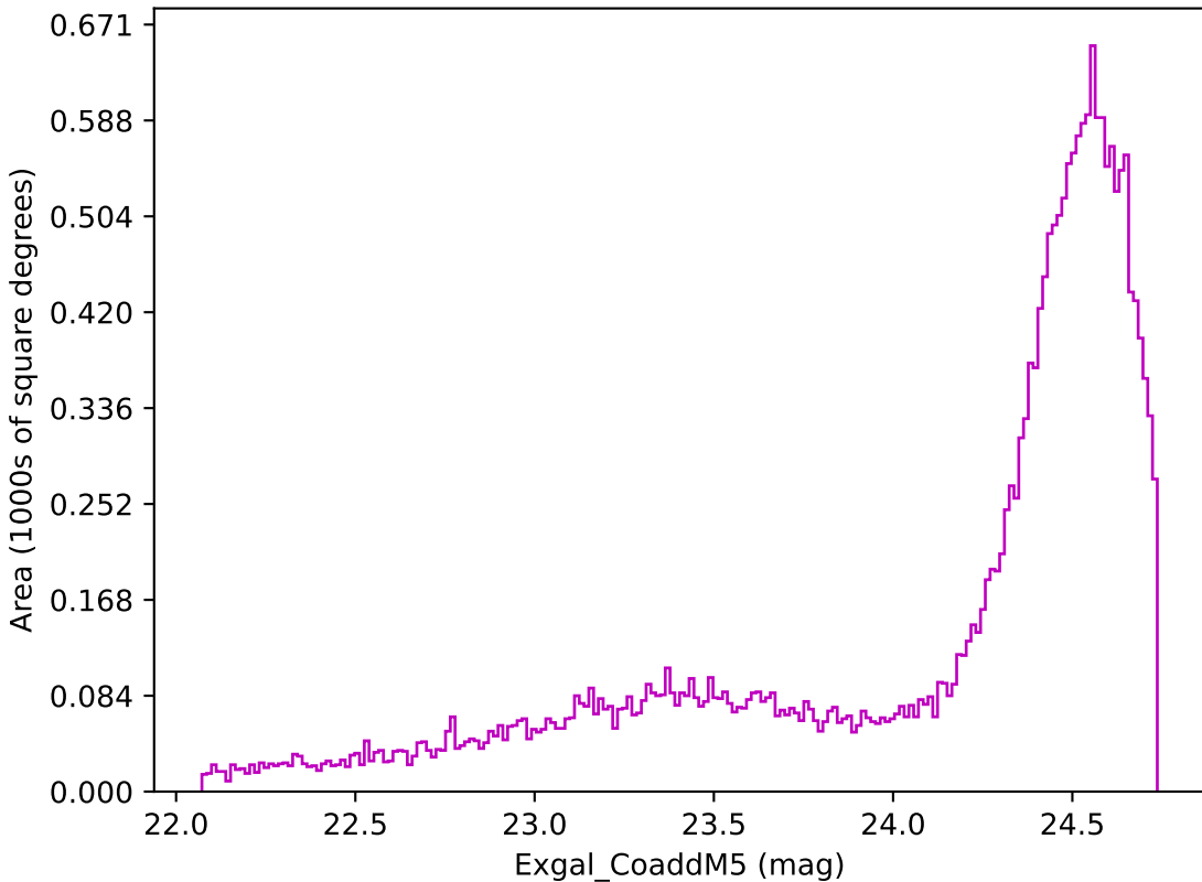
baseline_v3.3_10yrs Yr 1 z band: Exgal_CoaddM5
