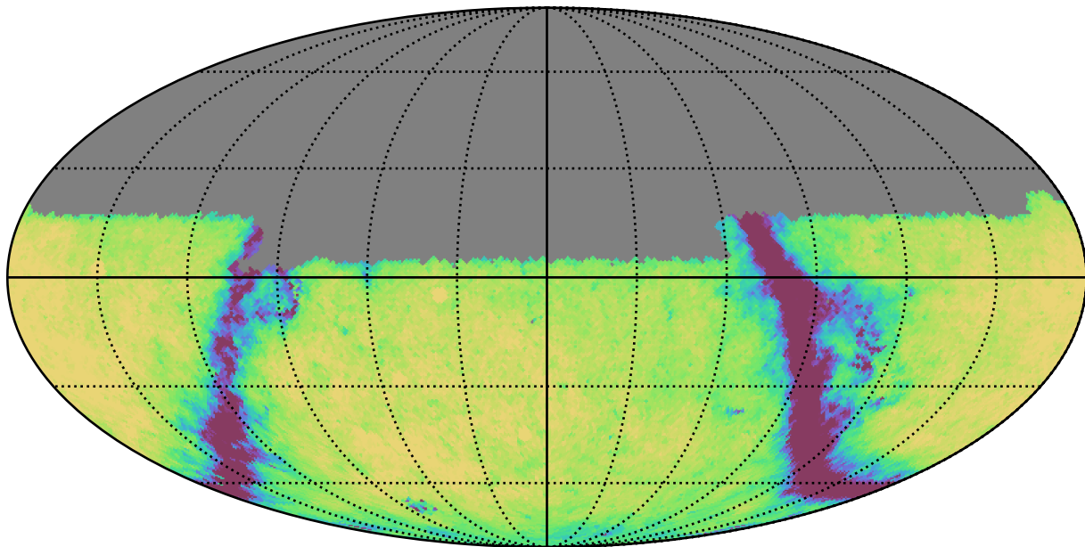
baseline_v3.3_10yrs Yr 1 u band: Exgal_CoaddM5
