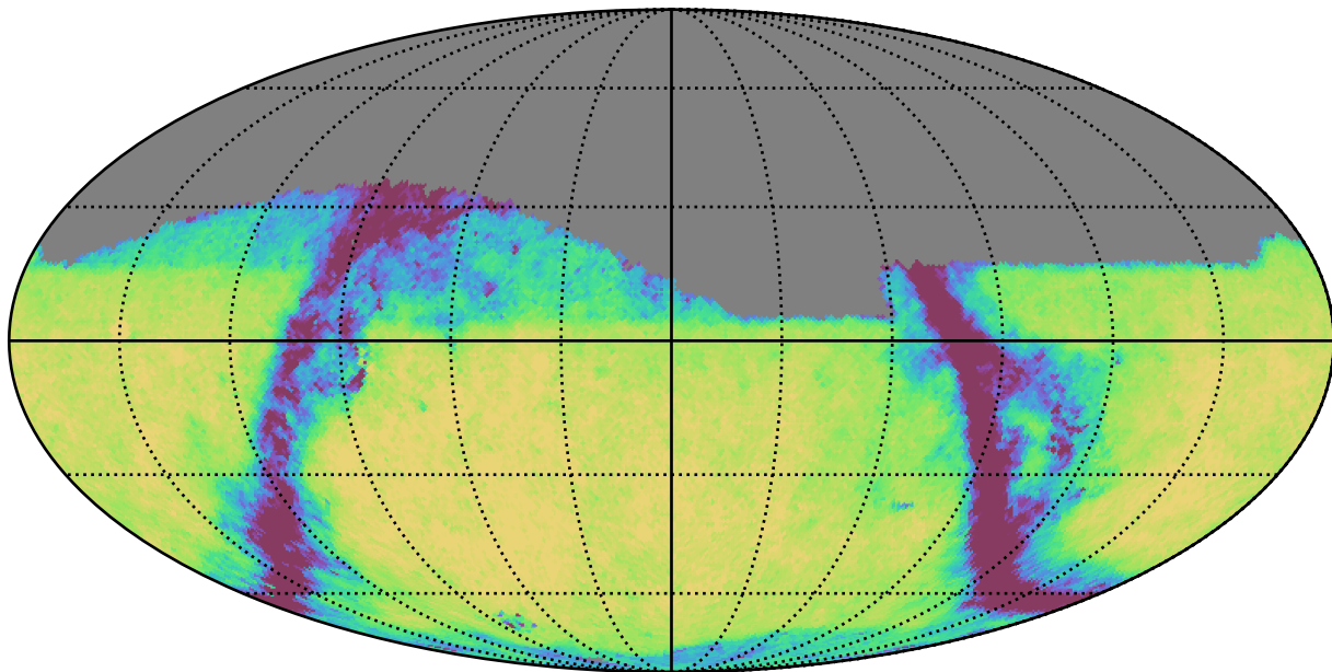
baseline_v3.3_10yrs Yr 1 r band: Exgal_CoaddM5
