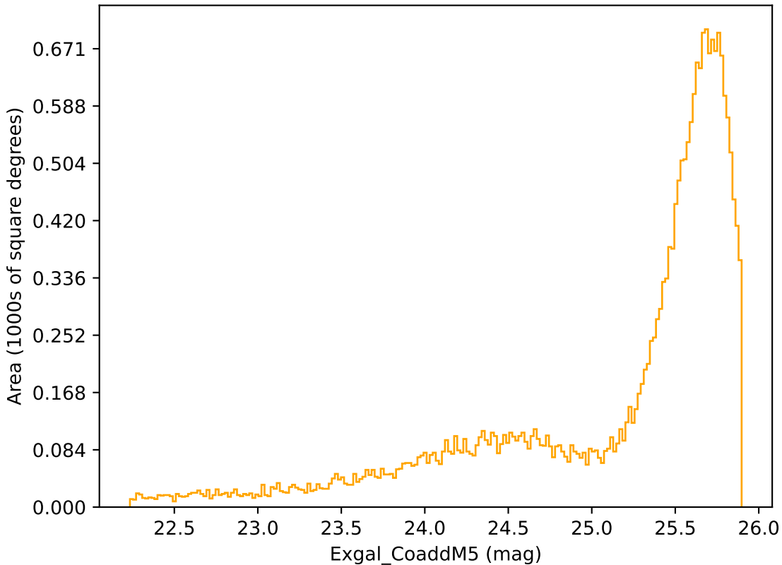
baseline_v3.3_10yrs Yr 1 r band: Exgal_CoaddM5
