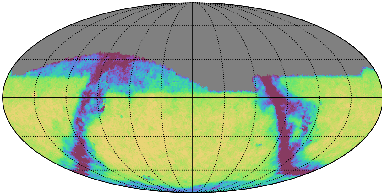
baseline_v3.3_10yrs Yr 1 i band: Exgal_CoaddM5
