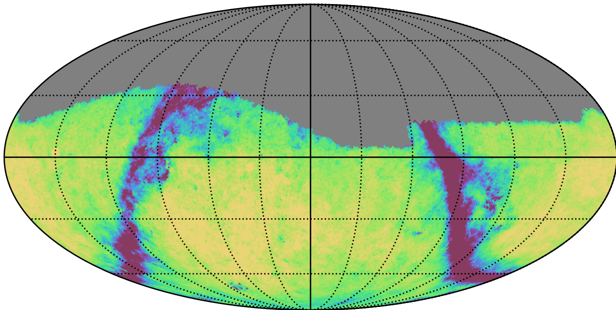
baseline_v3.3_10yrs Yr 1 g band: Exgal_CoaddM5
