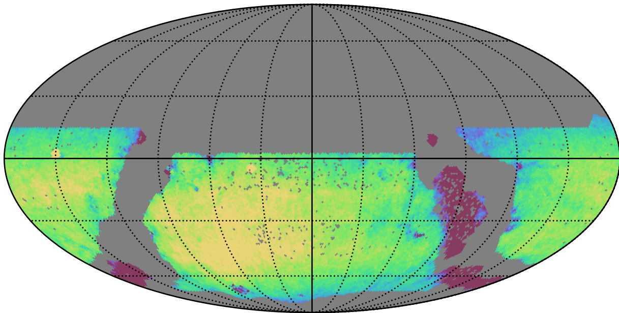
baseline_v3.3_10yrs WFD z band: Exgal_CoaddM5
