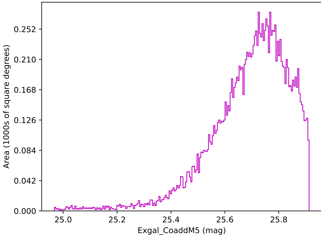
baseline_v3.3_10yrs WFD z band: Exgal_CoaddM5
