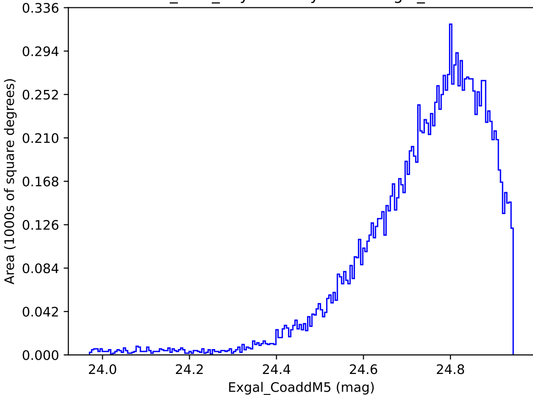
baseline_v3.3_10yrs WFD y band: Exgal_CoaddM5
