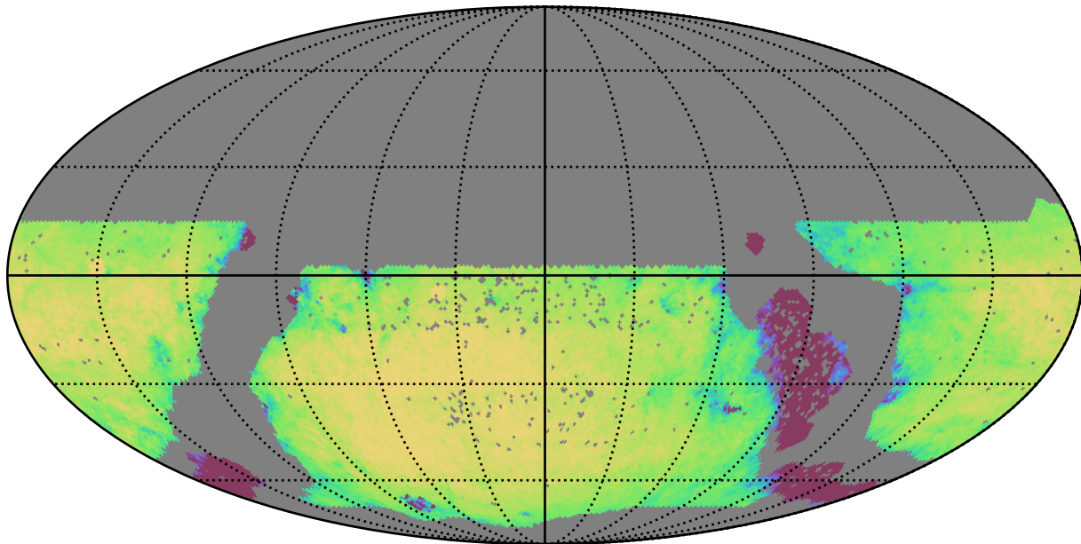
baseline_v3.3_10yrs WFD u band: Exgal_CoaddM5
