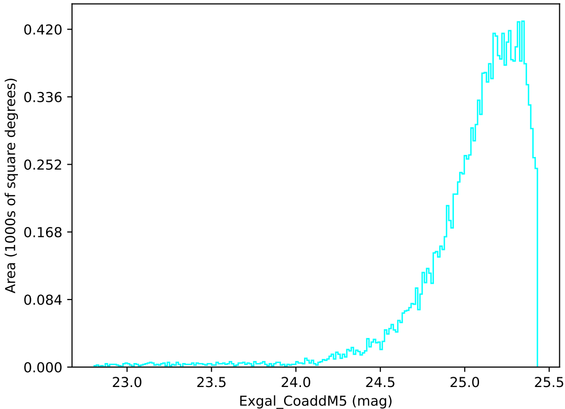
baseline_v3.3_10yrs WFD u band: Exgal_CoaddM5
