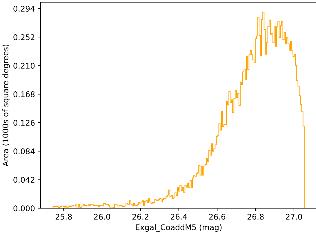
baseline_v3.3_10yrs WFD r band: Exgal_CoaddM5
