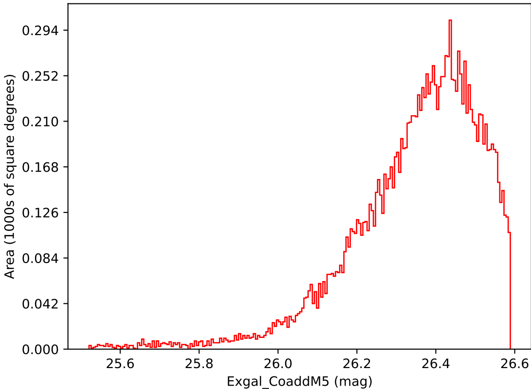
baseline_v3.3_10yrs WFD i band: Exgal_CoaddM5
