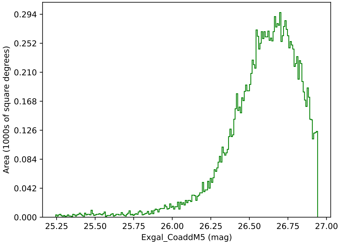
baseline_v3.3_10yrs WFD g band: Exgal_CoaddM5
