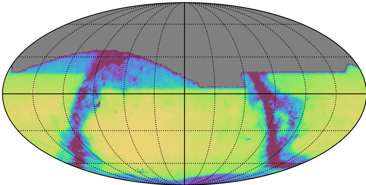
baseline_v3.3_10yrs All sky z band: Exgal_CoaddM5
