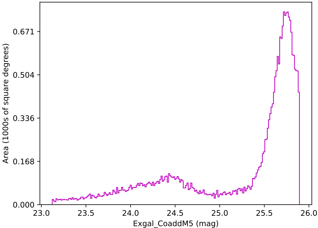
baseline_v3.3_10yrs All sky z band: Exgal_CoaddM5
