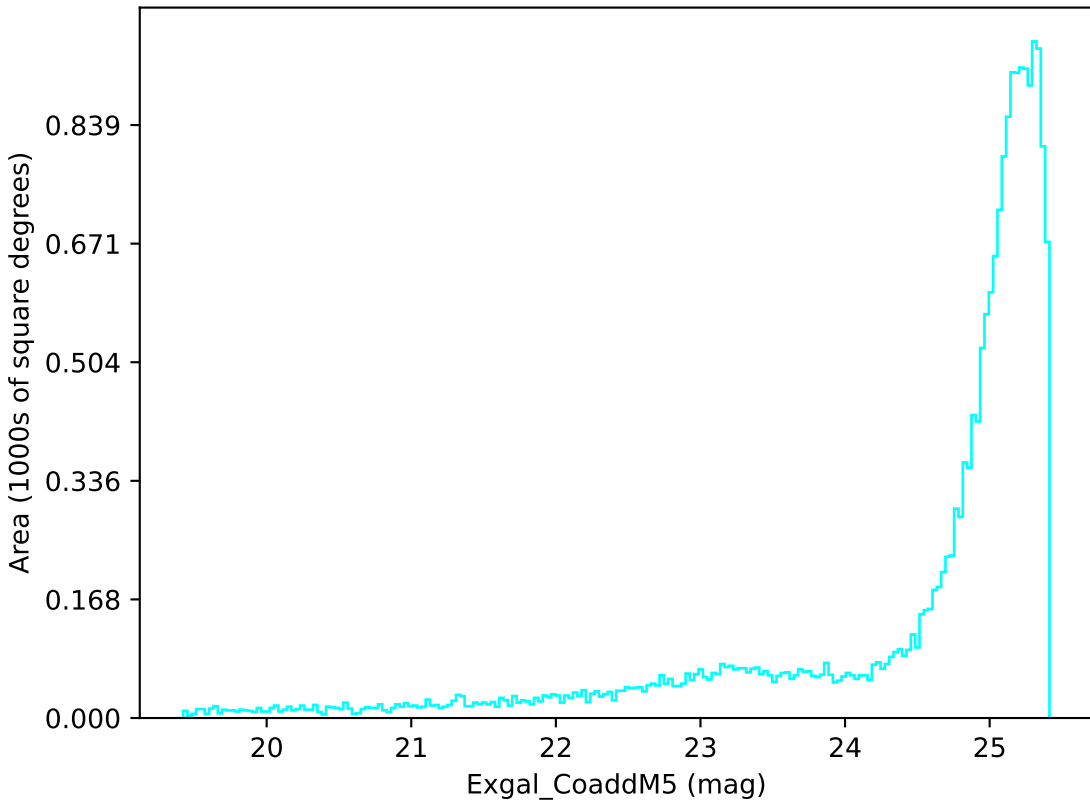
baseline_v3.3_10yrs All sky u band: Exgal_CoaddM5
