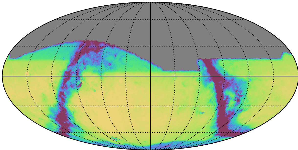
baseline_v3.3_10yrs All sky r band: Exgal_CoaddM5
