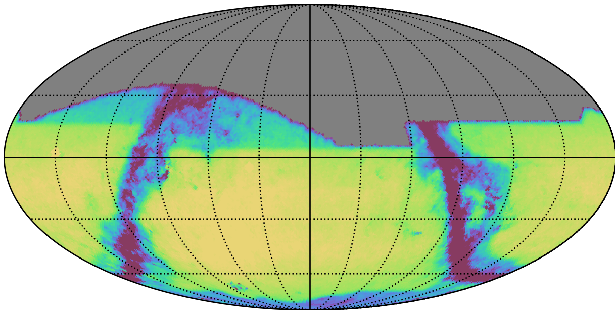
baseline_v3.3_10yrs All sky i band: Exgal_CoaddM5
