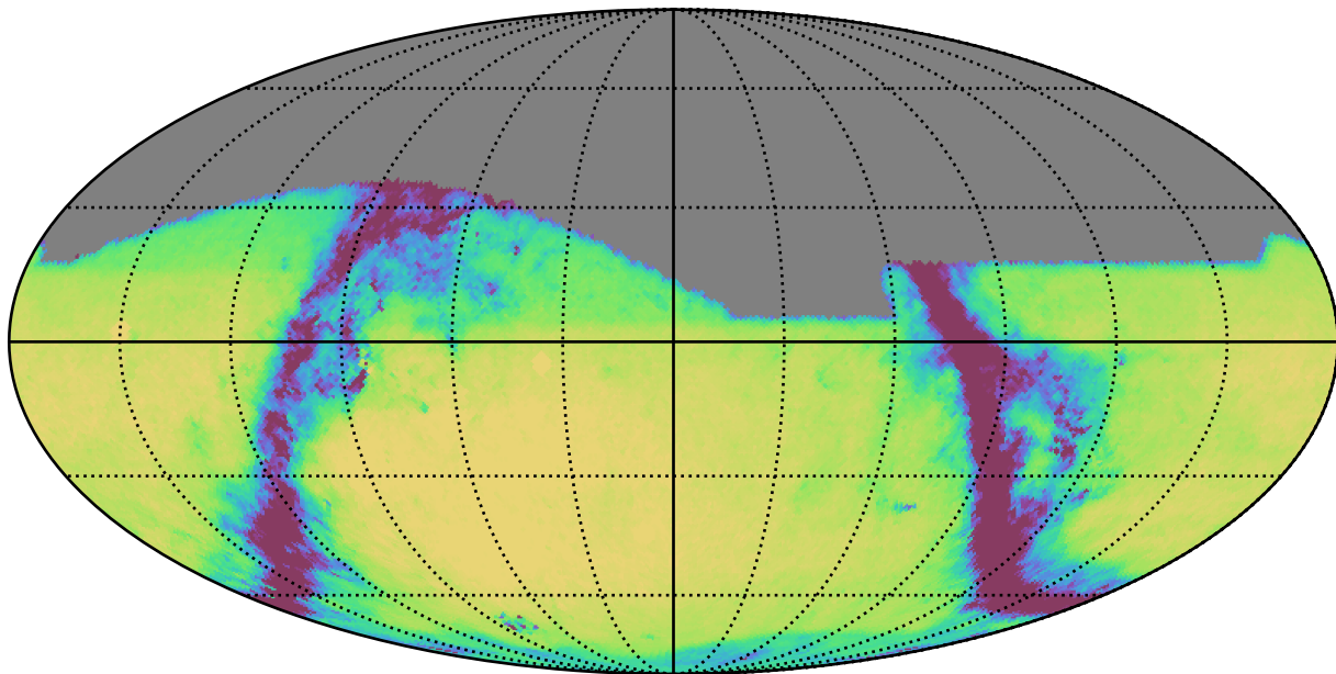
baseline_v3.3_10yrs All sky g band: Exgal_CoaddM5
