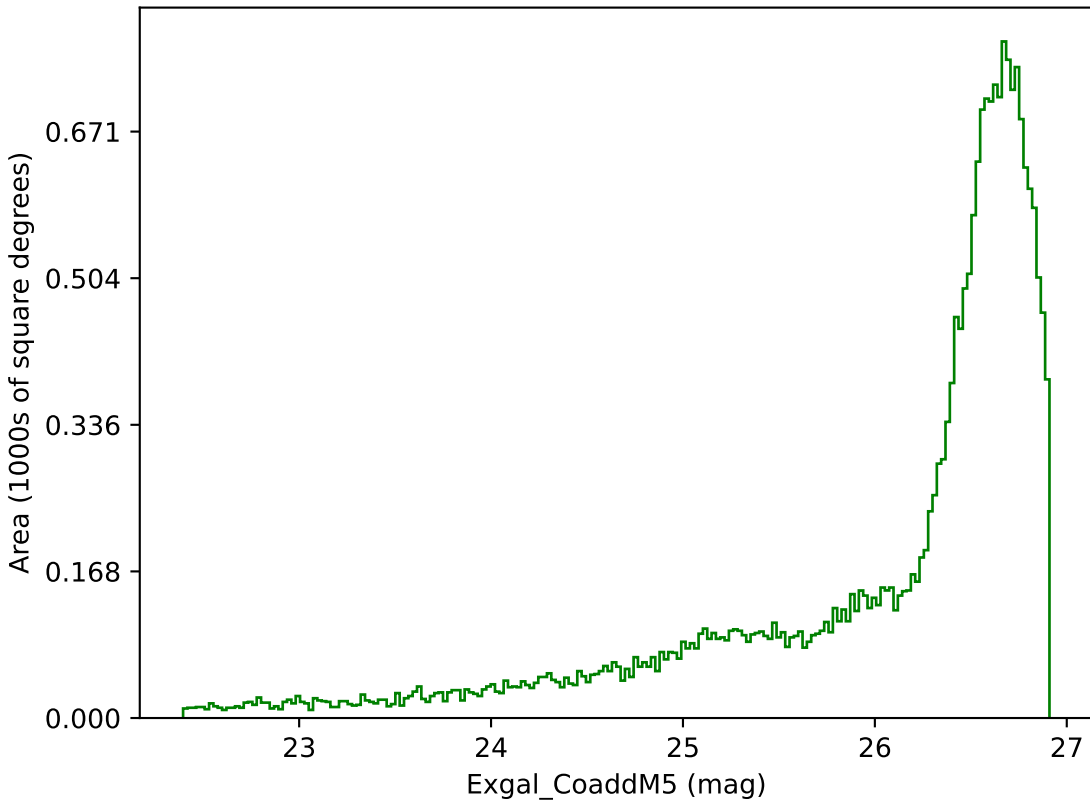
baseline_v3.3_10yrs All sky g band: Exgal_CoaddM5
