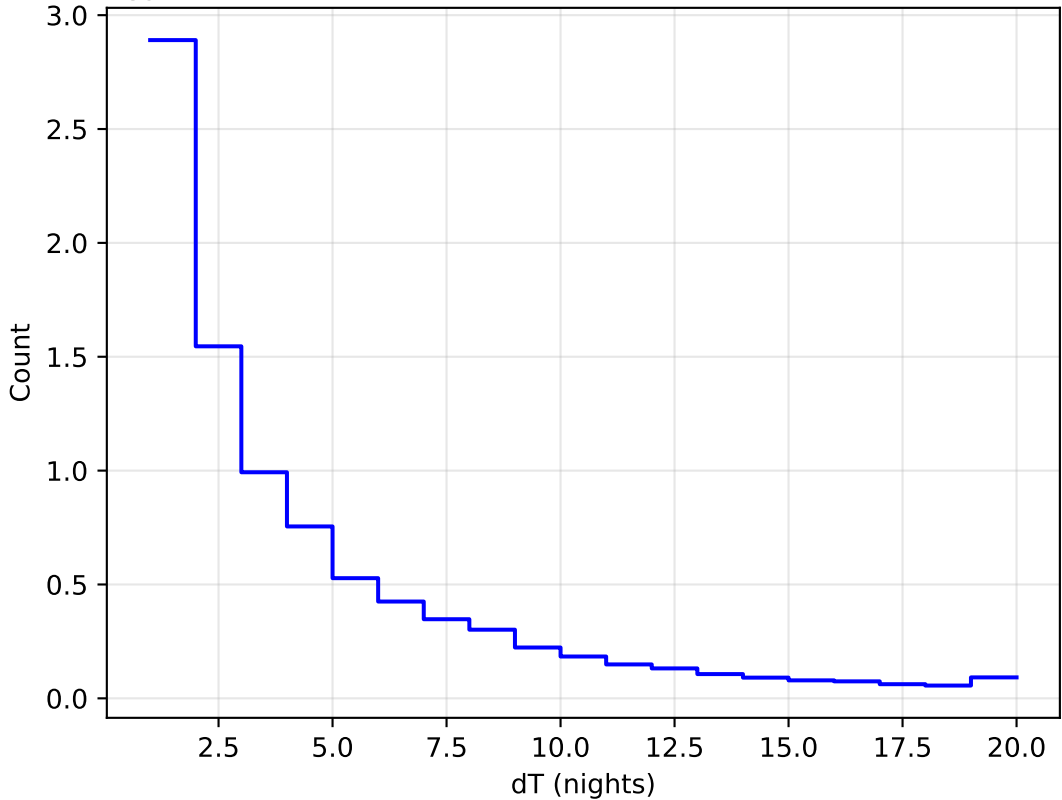
baseline_v3.3_10yrs All sky all bands: DeltaNight Histogram 1e6
