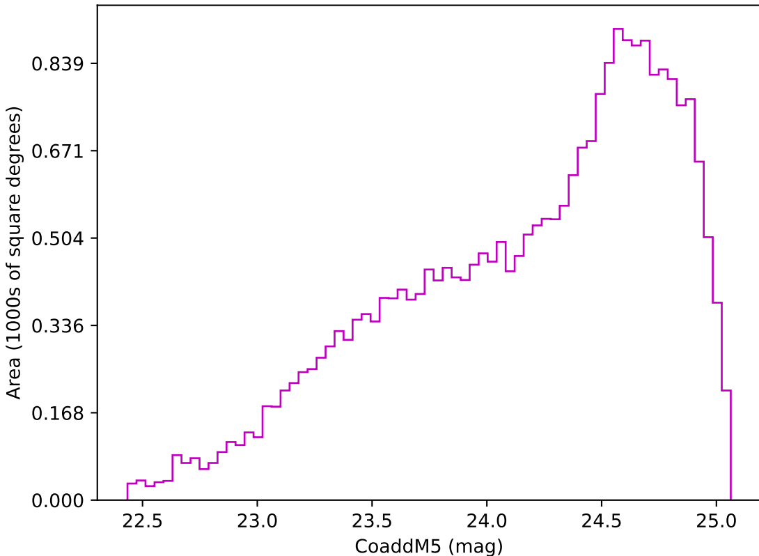
baseline_v3.3_10yrs Yr 3-4 z band: CoaddM5
