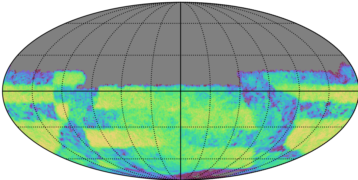
baseline_v3.3_10yrs Yr 3-4 y band: CoaddM5
