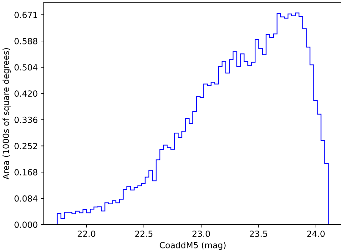
baseline_v3.3_10yrs Yr 3-4 y band: CoaddM5
