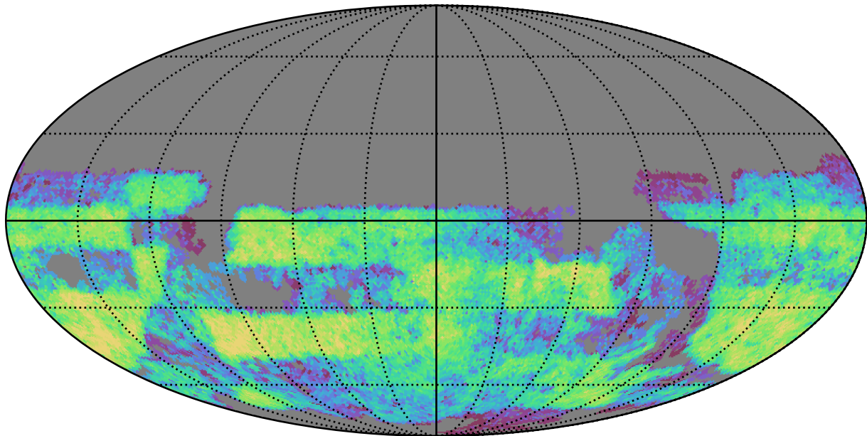
baseline_v3.3_10yrs Yr 3-4 u band: CoaddM5
