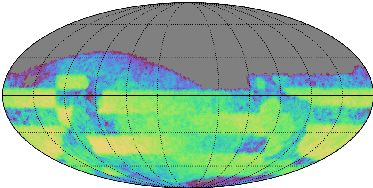
baseline_v3.3_10yrs Yr 3-4 i band: CoaddM5
