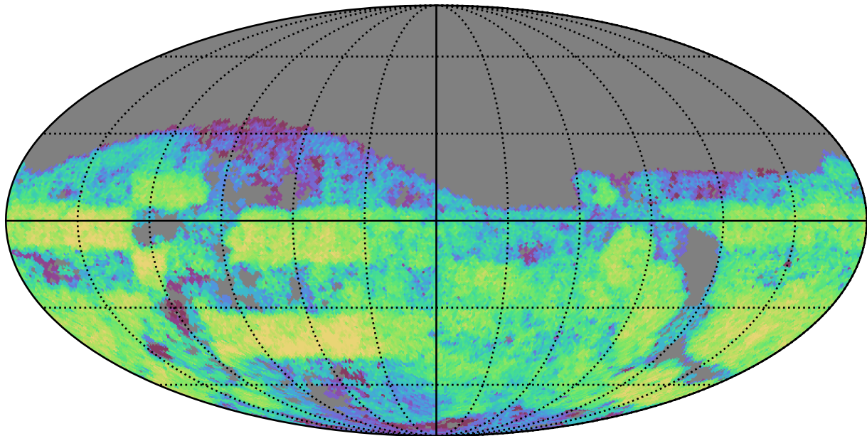
baseline_v3.3_10yrs Yr 3-4 g band: CoaddM5
