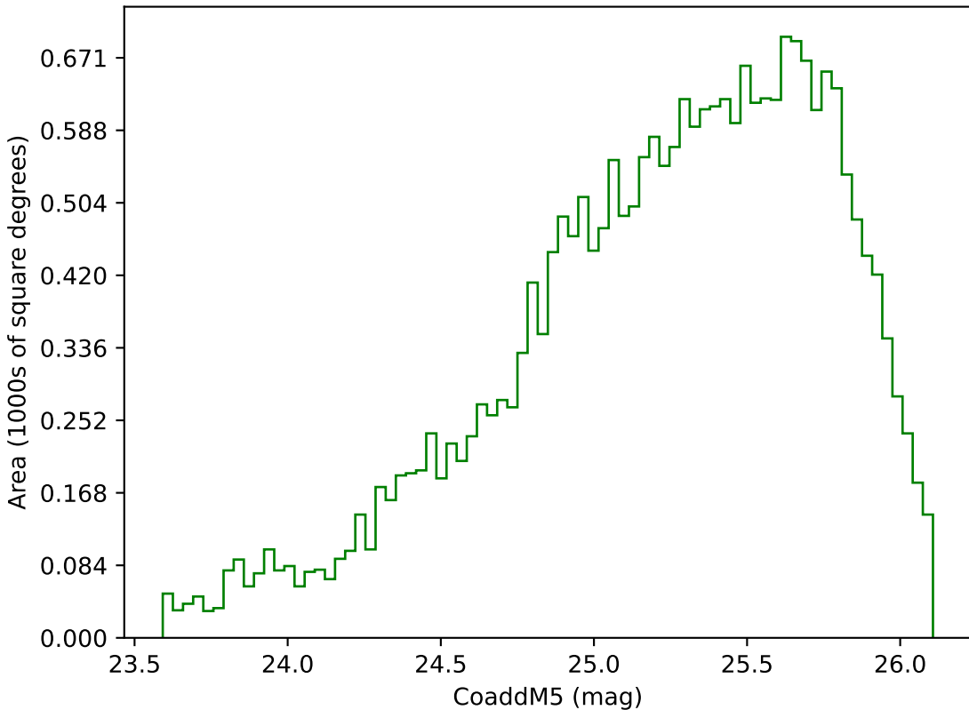
baseline_v3.3_10yrs Yr 3-4 g band: CoaddM5
