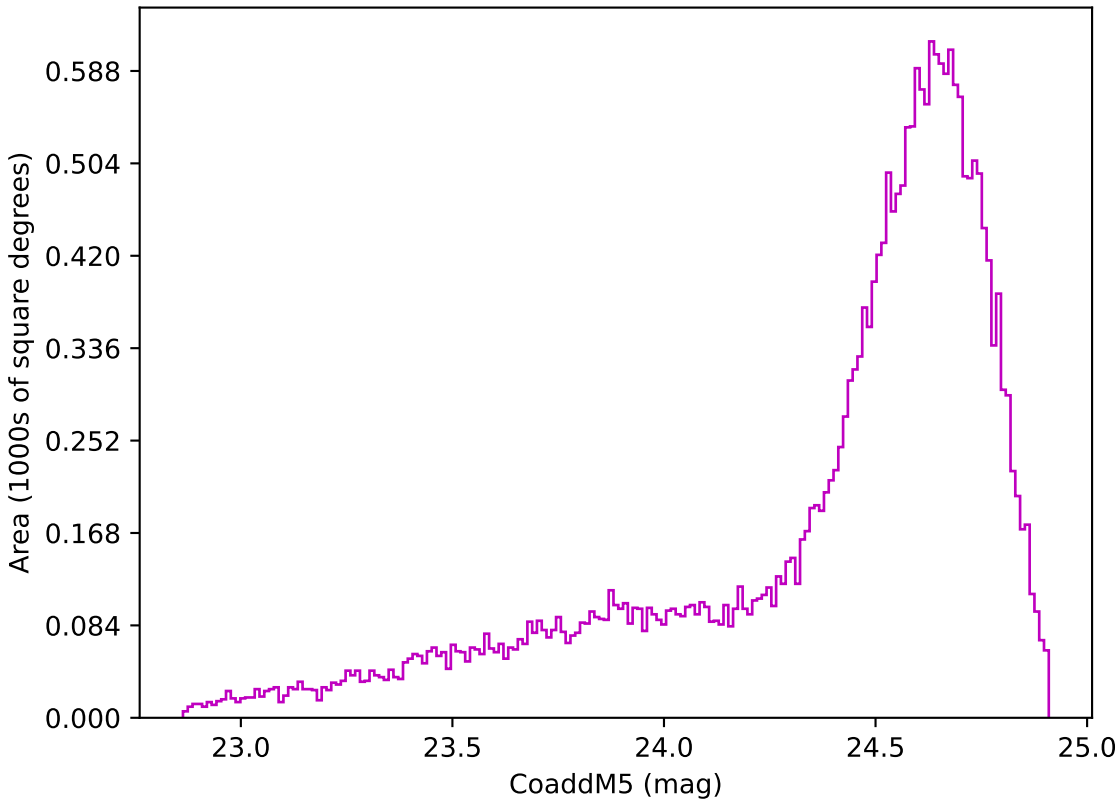
baseline_v3.3_10yrs Yr 1 z band: CoaddM5
