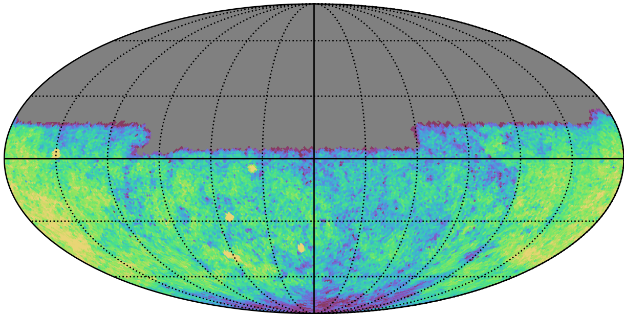
baseline_v3.3_10yrs Yr 1 u band: CoaddM5
