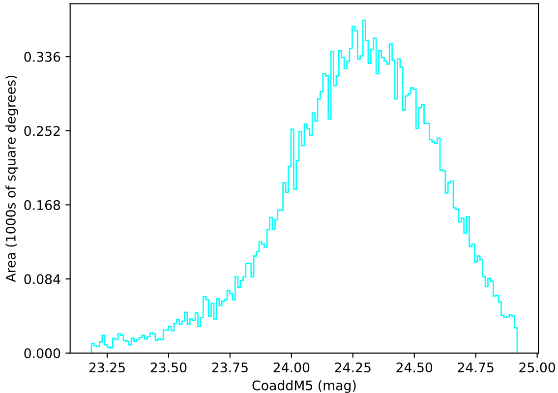
baseline_v3.3_10yrs Yr 1 u band: CoaddM5
