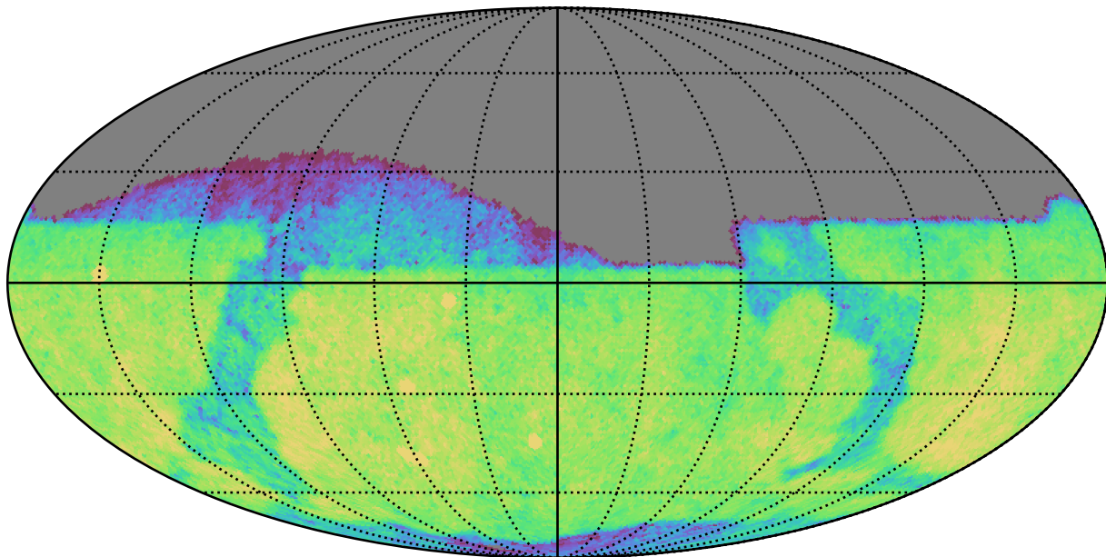
baseline_v3.3_10yrs Yr 1 r band: CoaddM5
