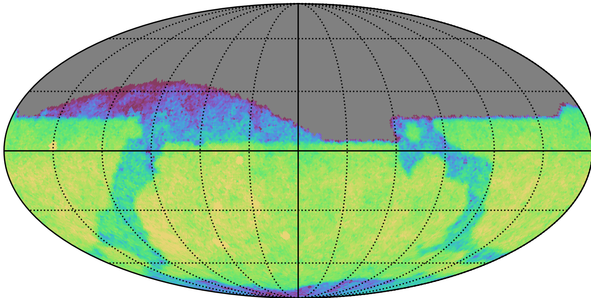
baseline_v3.3_10yrs Yr 1 i band: CoaddM5
