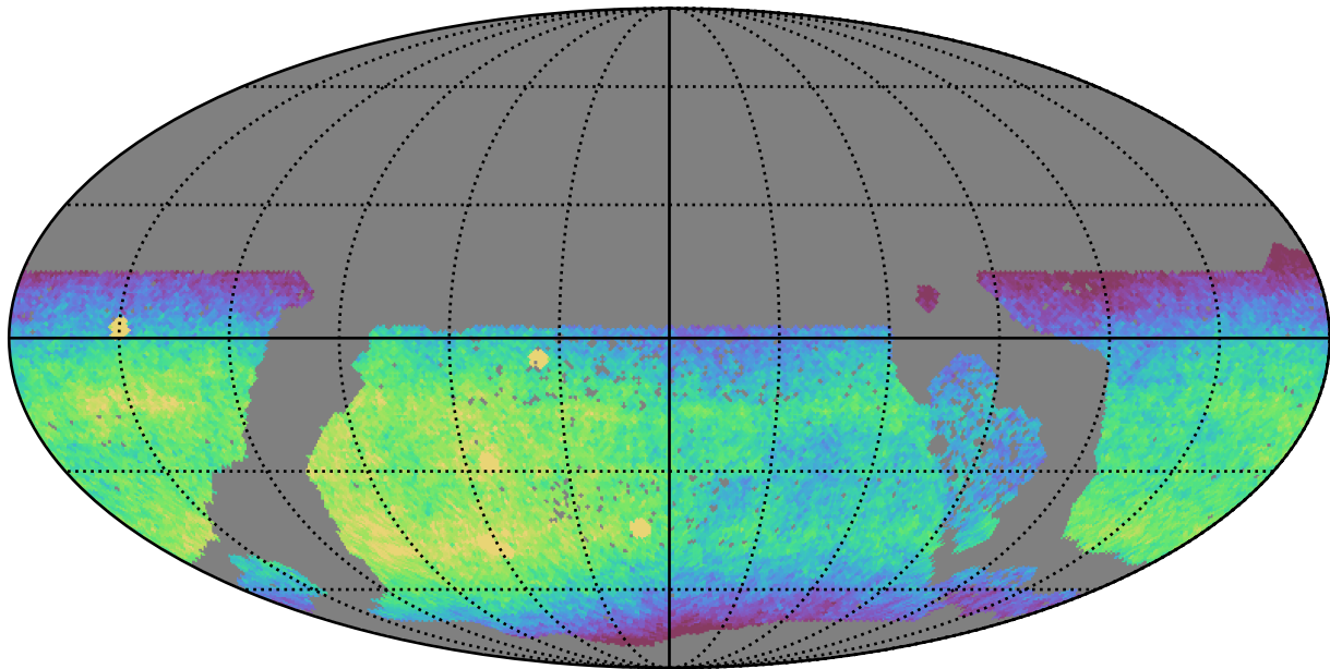
baseline_v3.3_10yrs WFD z band: CoaddM5
