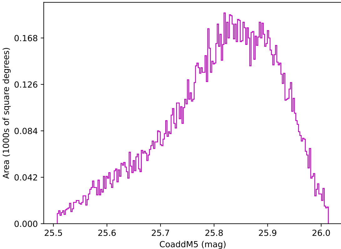
baseline_v3.3_10yrs WFD z band: CoaddM5
