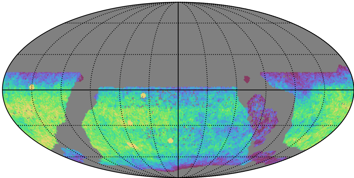
baseline_v3.3_10yrs WFD u band: CoaddM5
