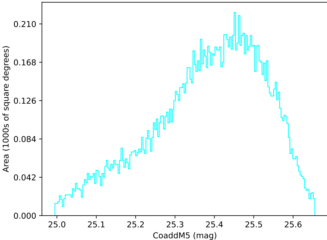
baseline_v3.3_10yrs WFD u band: CoaddM5
